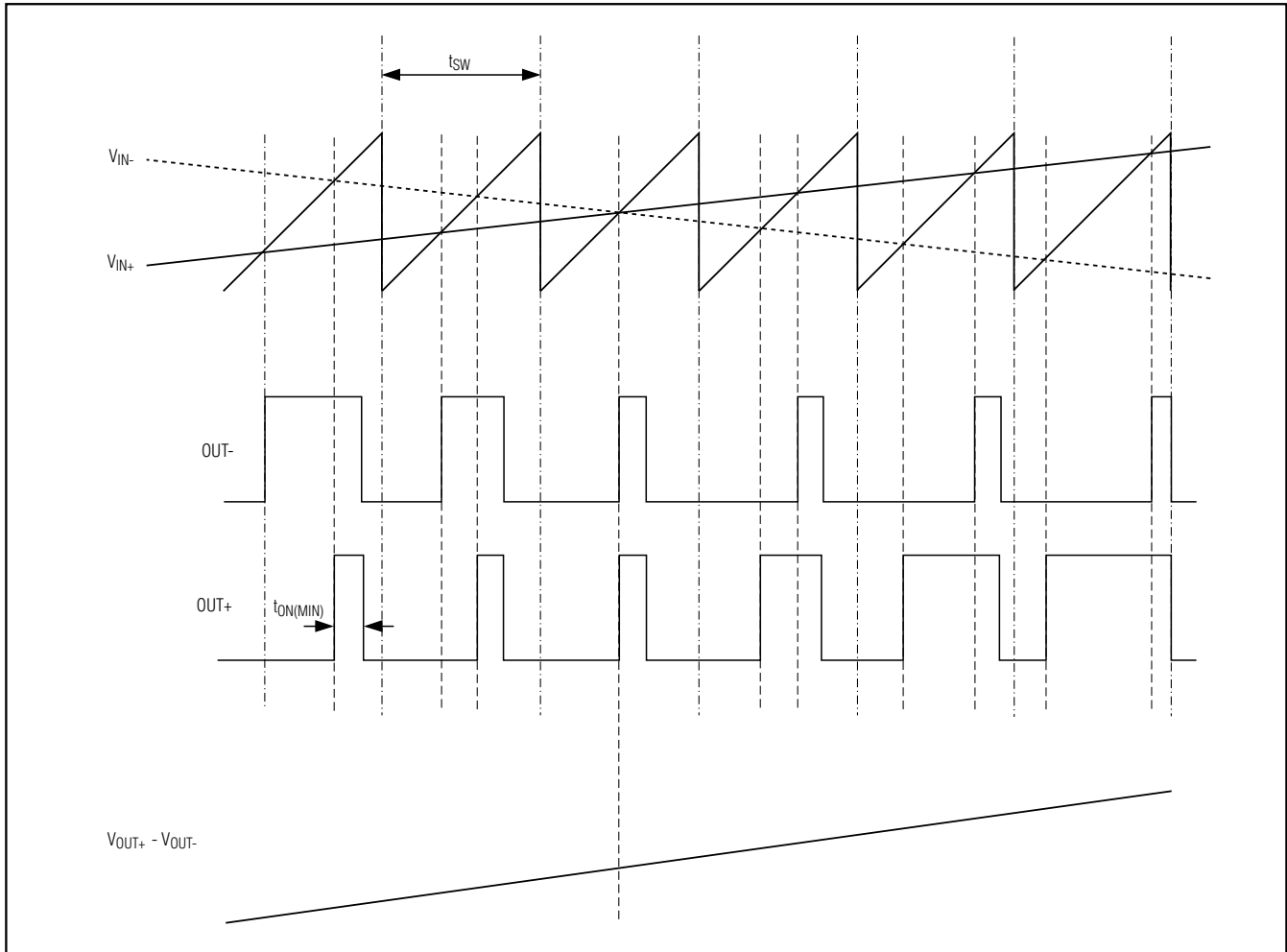
Figure 1. MAX9759 Outputs with an Input Signal Applied
