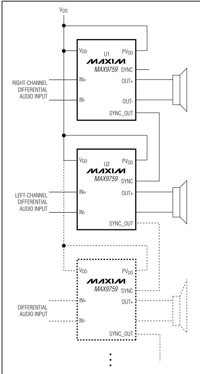
Figure 7. Master-Slave Configuration
